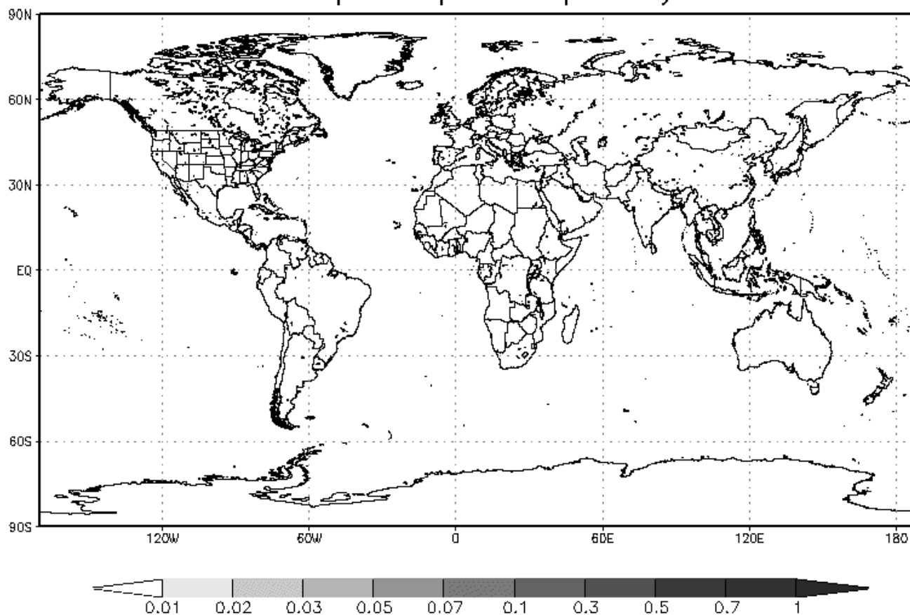
BC Absorption Optical Depth May 14th
